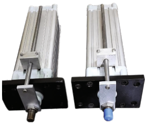
Magnetic Cylinder Non Rotating
